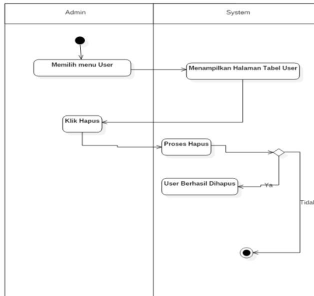
Figure 5. Activity Diagram when admin manage use accounts
