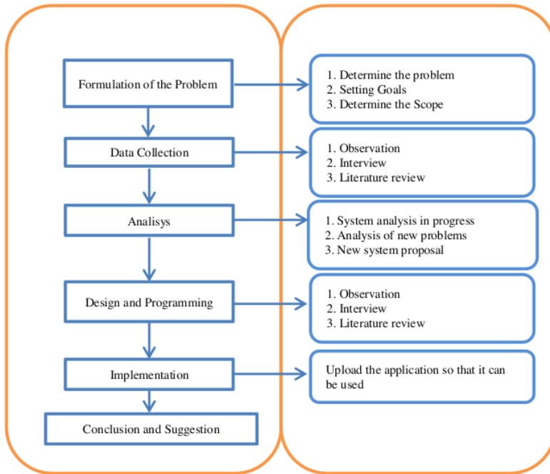
Figure 1. Research Method
