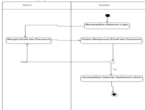
Figure 4. Activity diagram for login process
