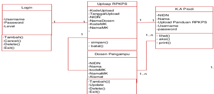
Gambar 4. Class Diagram
