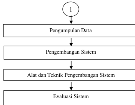
Gambar 1. Metode penelitian
