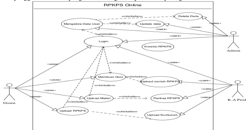
Gambar 2. Usecase Diagram
