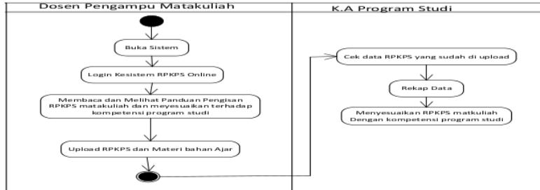
Gambar 3. Activity Diagram
