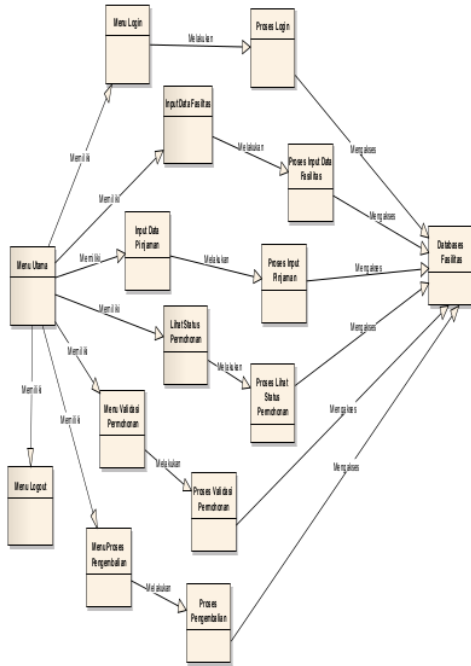
Gambar 8 Class Diagram
