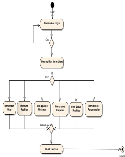
Gambar 1 Bisnis Proses Model
