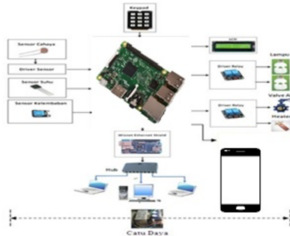
Gambar 6. Diagram Blok Sistem Greenhouse.
