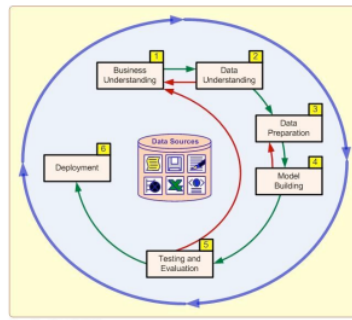
Gambar 1. Model CRISP-DM
